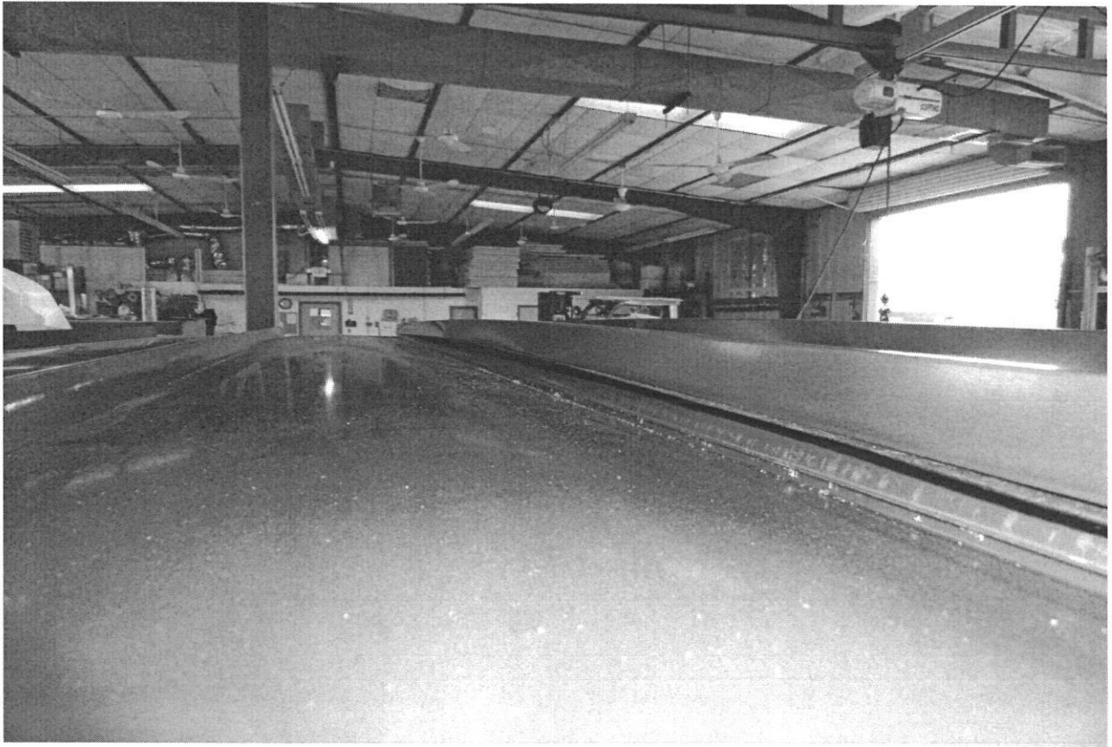
TEST B FAILURE, PANEL SEAMS DISENGAGED
