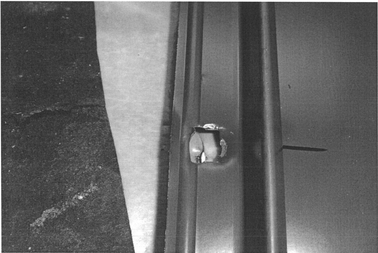
TEST A FAILURE, FASTENER FLANGE TORE AROUND FASTENER HEAD
